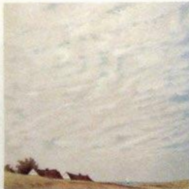
6. Alto-cumulus.
