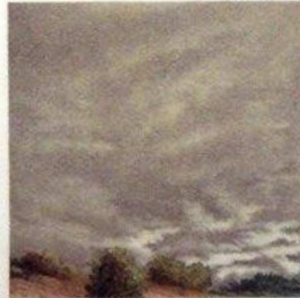
7. Strato-cumulus.
